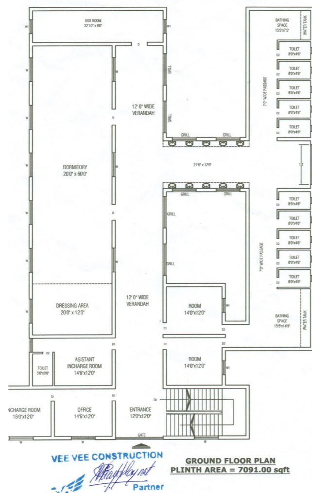
PROPOSED PLAN OF A TRIBAL GIRLS HOSTEL FOR ST. ALOYSIUS SECONDARY SCHOOL AT HIRALOI DIST- SAMBALPUR, STATE - ODISHA
